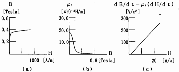
Fig. 3. Parameters \mu , \mu_r and s of the Chua type model for a ferrite (TDK H5c2); (a) permeability \mu(=B/H) , (b) reversible permeability \mu_r vs. B curve, where B is a bias flux density, (c) (dB/dt) - \mu_r(dH/dt) vs. H curve, where s = [(dB/dt) - \mu_r(dH/dt)]/H .
